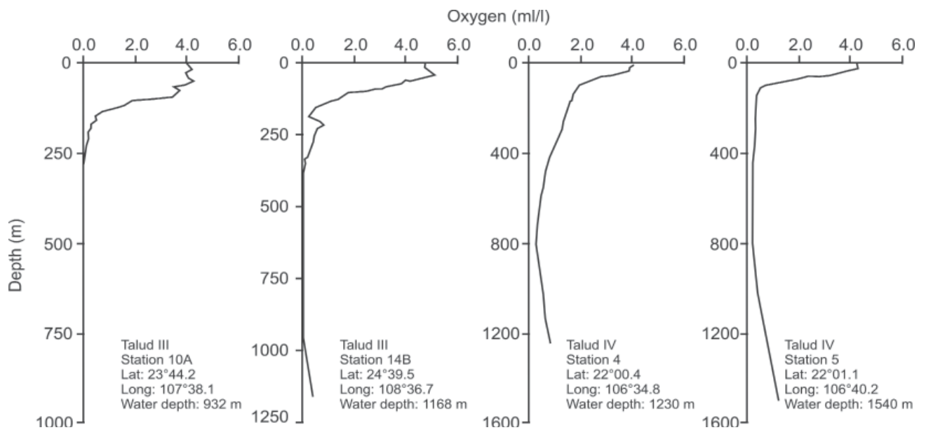
Figure 1. Some examples of vertical distribution of the dissolved oxygen concentration in the sampled area (Source: Hendrickx, 2001).
